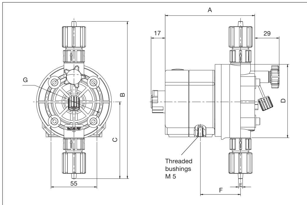
Dimension sheet PNDb PVC (dimensions in mm)
