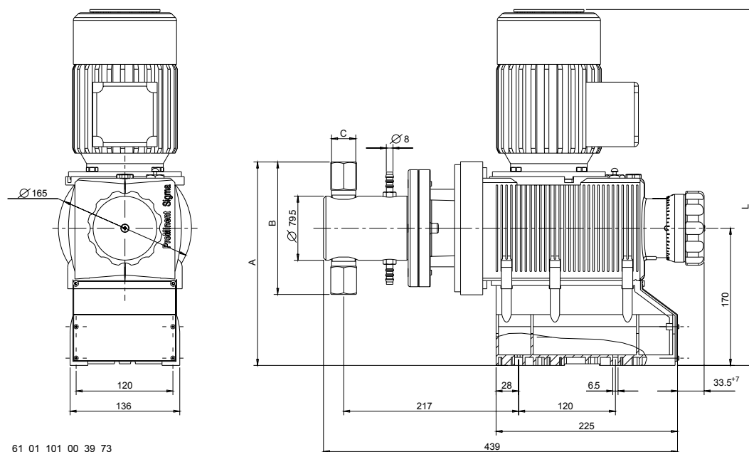
Fig. 1: Dimensional drawing Sigma SBKa - dimensions in mm
