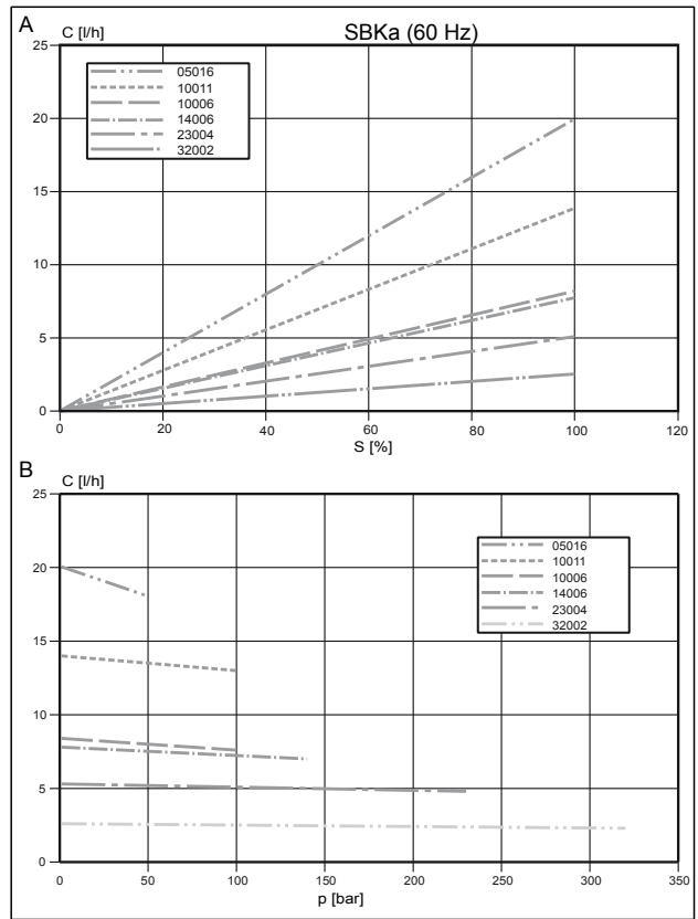
Fig. 2: A) Capacity C at minimum back pressure dependent on the stroke length s. B) Capacity C dependent on the back pressure p.
