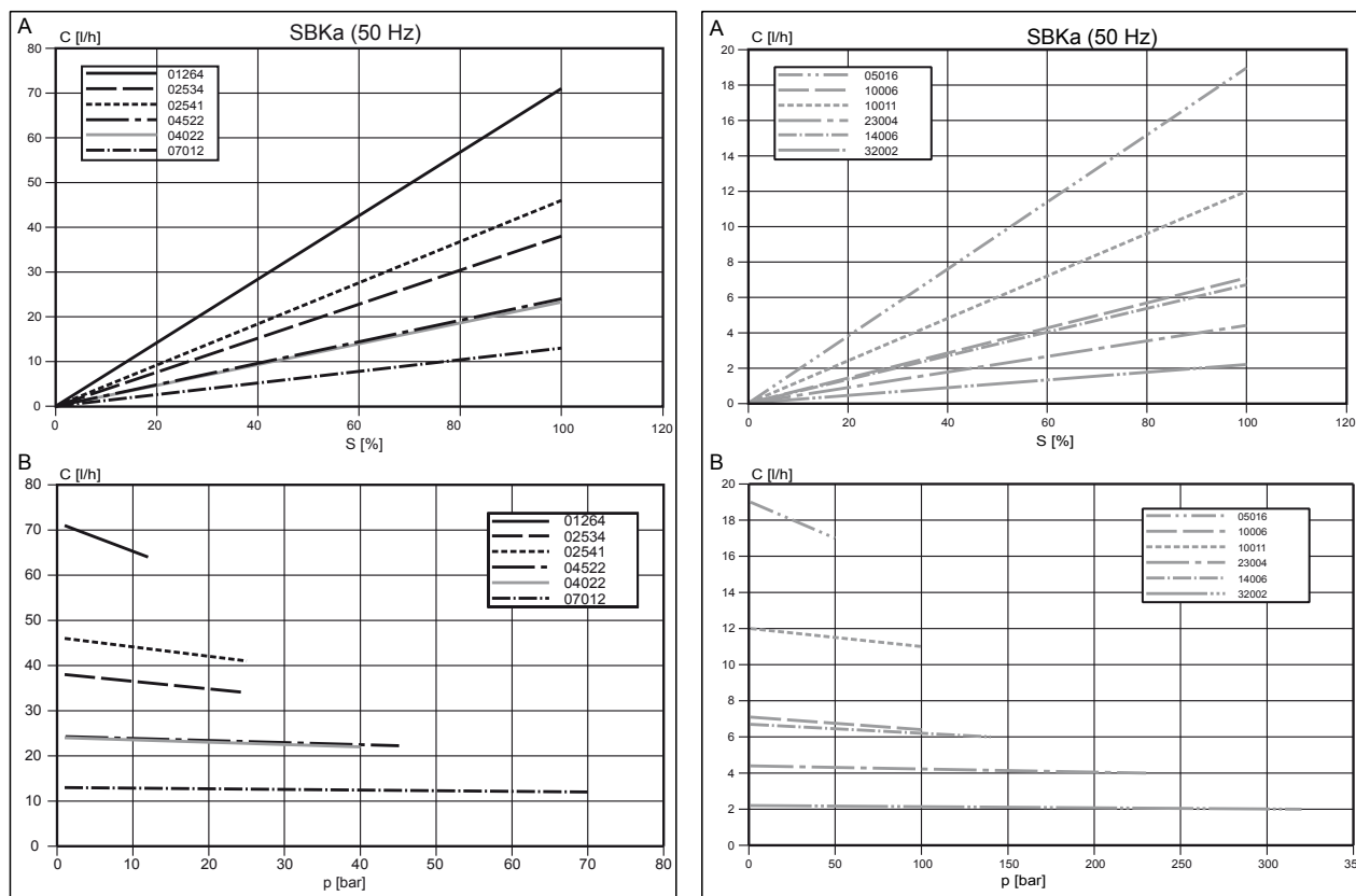
Fig. 1: A) Capacity C at minimum back pressure dependent on the stroke length s . B) Capacity C dependent on the back pressure p .
