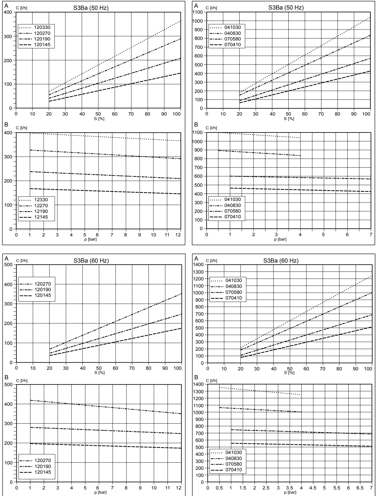
Fig. 1: A) Capacity C at minimum back pressure dependent on the stroke length s . B) Capacity C dependent on the back pressure p .
