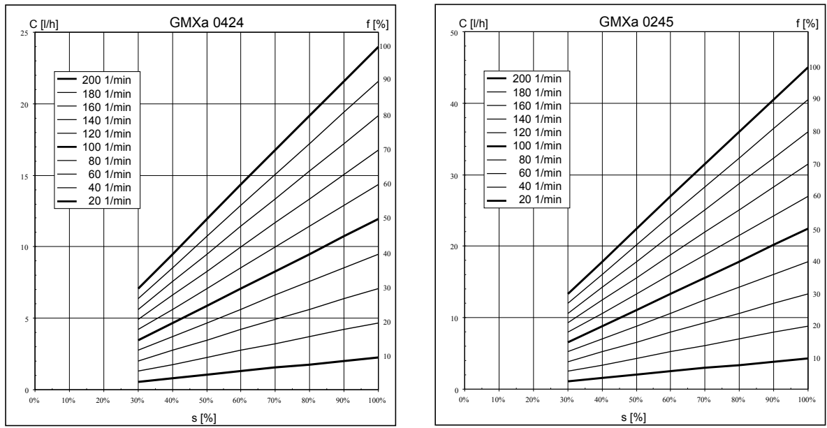
Fig. 3: Capacity C at medium back pressure depending on the stroke length s for different stroke rates f
