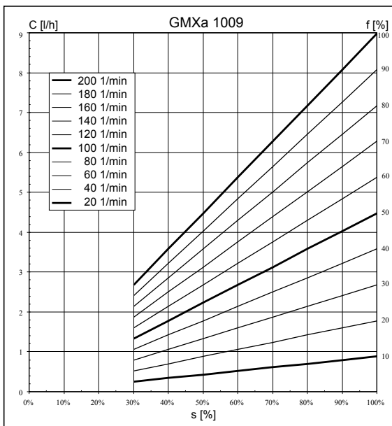
Fig. 2: Capacity C at medium back pressure depending on the stroke length s for different stroke rates f
