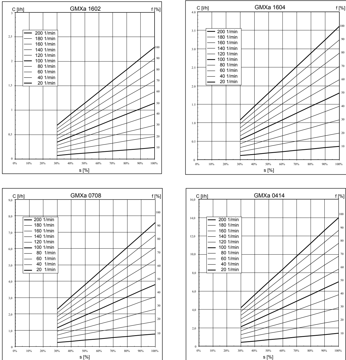
Fig. 1: Capacity C at medium back pressure depending on the stroke length s for different stroke rates f
