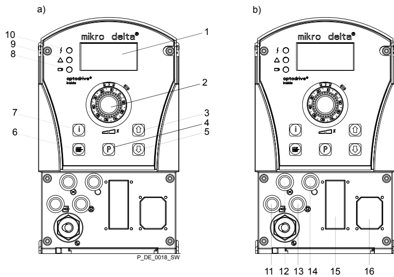
Fig. 4: a) Displays delta and keys, b) Electrical control connections
