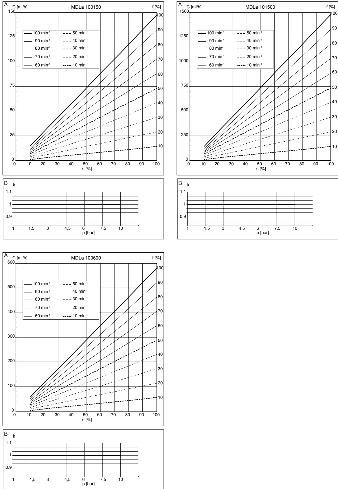
Fig. 33: A) Metering capacity C at medium back pressure dependent on the stroke length s for different stroke rates f . - B) Corresponding correction factors k dependent on the back pressure p .
