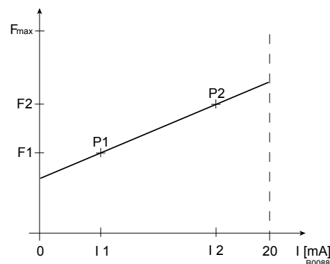
Fig. 21: Rate(frequency)-Current Diagram for Linear control
