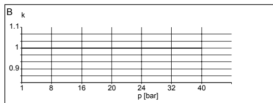
Fig. 34: A) Metering capacity C at medium back pressure dependent on the stroke length s for different stroke rates f . - B) Corresponding correction factors k dependent on the back pressure p .
