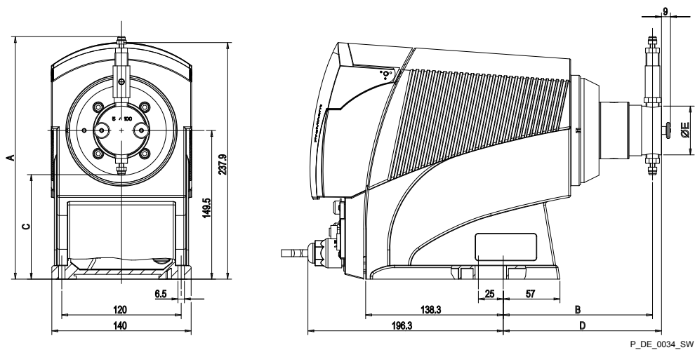
Fig. 32: Dimensions sheet delta ® MDL, material versions TT and SS - dimensions in mm
