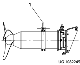
Lifting tackle
