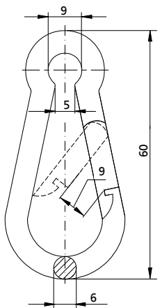
Dimensions of carabine hook [mm]
