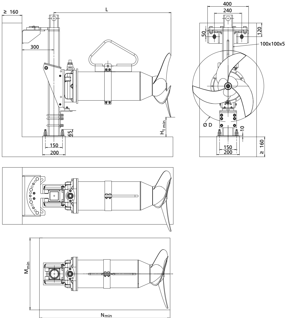
Installation with accessories set 22 - Amamix 400 (size 4135 only) / 600
