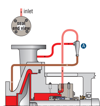
A - cyclone separator
