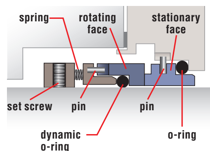
Component pusher seal
