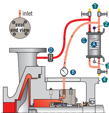
A - cooling coils B - temperature indicator C - cooler D - orifice 1 - vents, normally closed 2 - cooling out 3 - cooling in 4 - drain, normally closed
